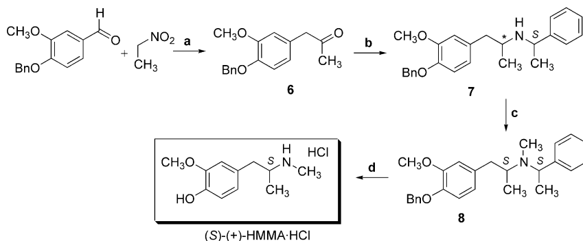
Scheme 3. Synthesis of enantiomerically enriched ( S )-HMMA·HCl. a: 1) \text{CH}_3\text{CO}_2\text{NH}_4 ; 2) Fe, \text{HCl}\cdot\text{H}_2\text{O} ; b: ( S )- \alpha -methylbenzylamine, \text{NaBH}_4 CN; c: 1) \text{CH}_3\text{L} , \text{Na}_2\text{CO}_3 ; 2) chromatography separation; d: 1) \text{HCl} ; 2) \text{H}_2 , Pd-C, MeOH.
